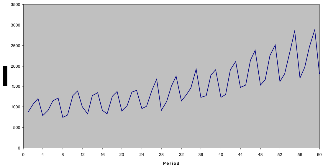
Figure 1. Time Series Used for Example Problem
